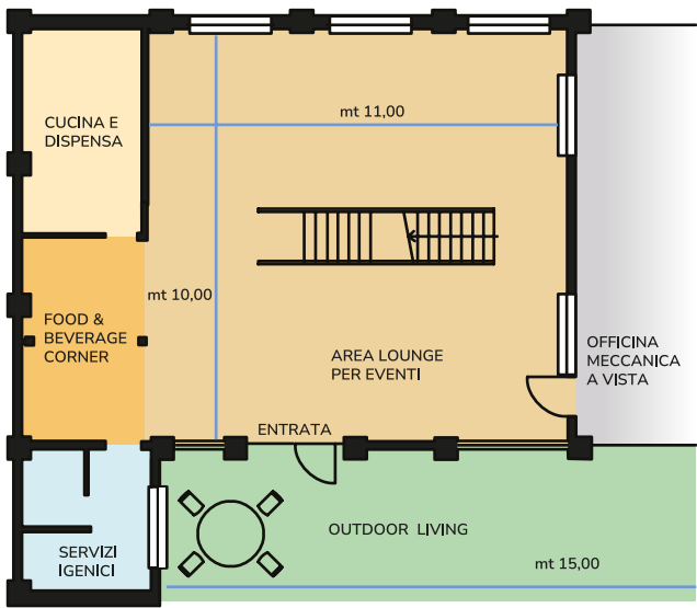
PIANO TERRA
